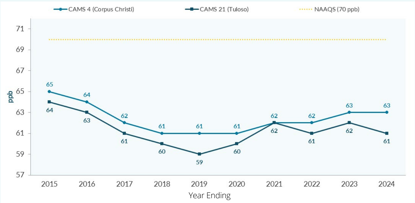
OZONE DESIGN VALUE TREND VS. NAAQS (3-Year Rolling Average of Annual 4th-Highest Reading)
